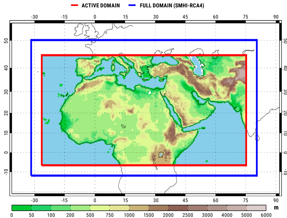
FIGURE 17: CORDEX-MENA Domain
